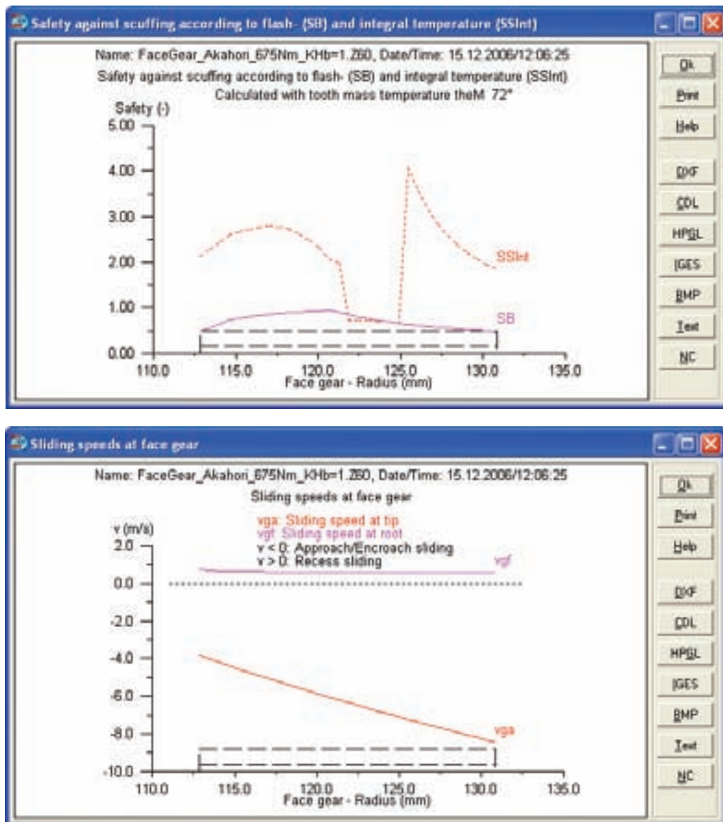
Figure 7 (Top & Bottom)—Scoring pitting safety factor against flash and integral temperature and speed at tip and root. Geometry of the face gear corresponds to the test gear of Akahori (Ref. 2).
